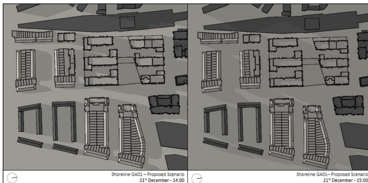
Figure 76 - Overshadowing image on December 21st at 2 p.m. and 3 p.m.
