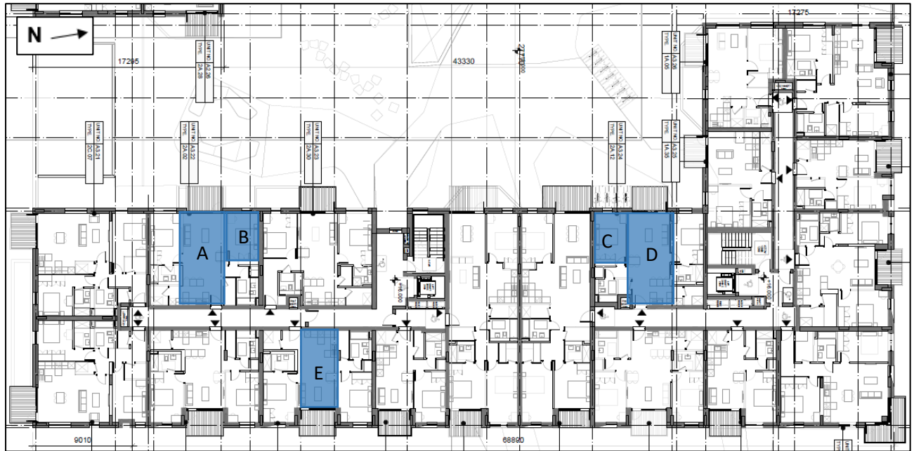
Figure 17 - Block A3 Level 02 - Assessed Rooms
