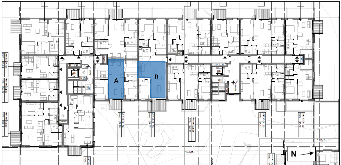
Figure 8 - Block A1 Level 03 - Assessed Rooms
