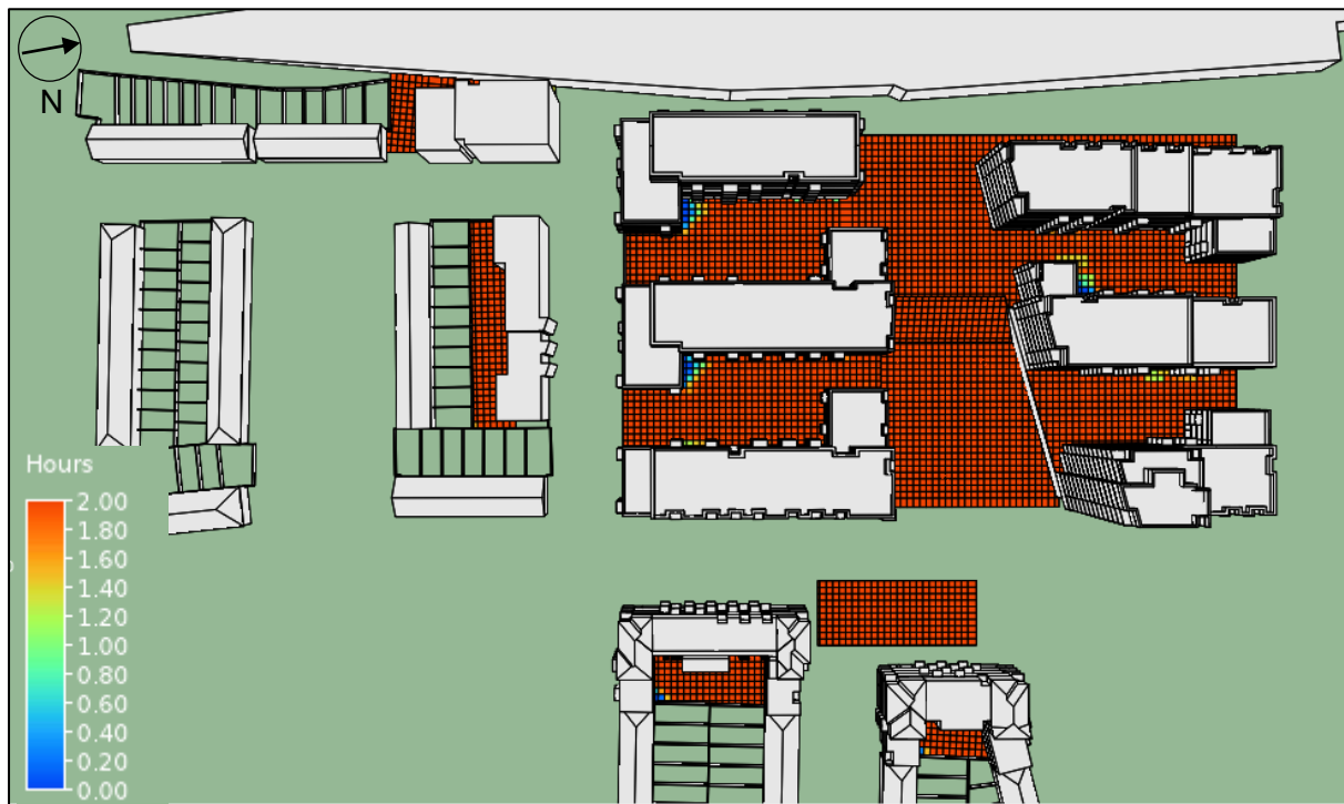
Figure 81 – Sunlight Analysis May 21 st
