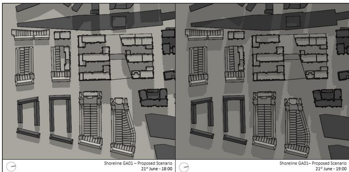
Figure 73 - Overshadowing image on June 21st at 6 p.m. and 7 p.m.
