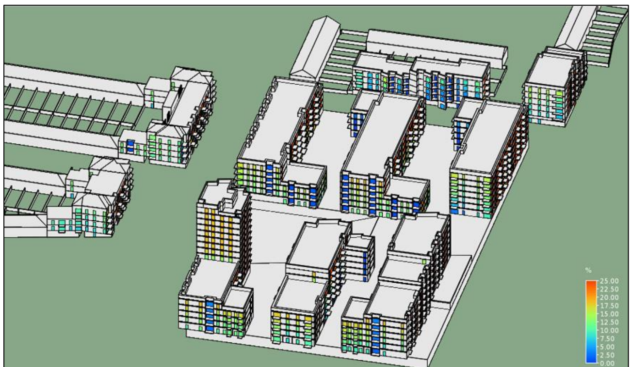
Figure 56 - APSH – North Elevation
