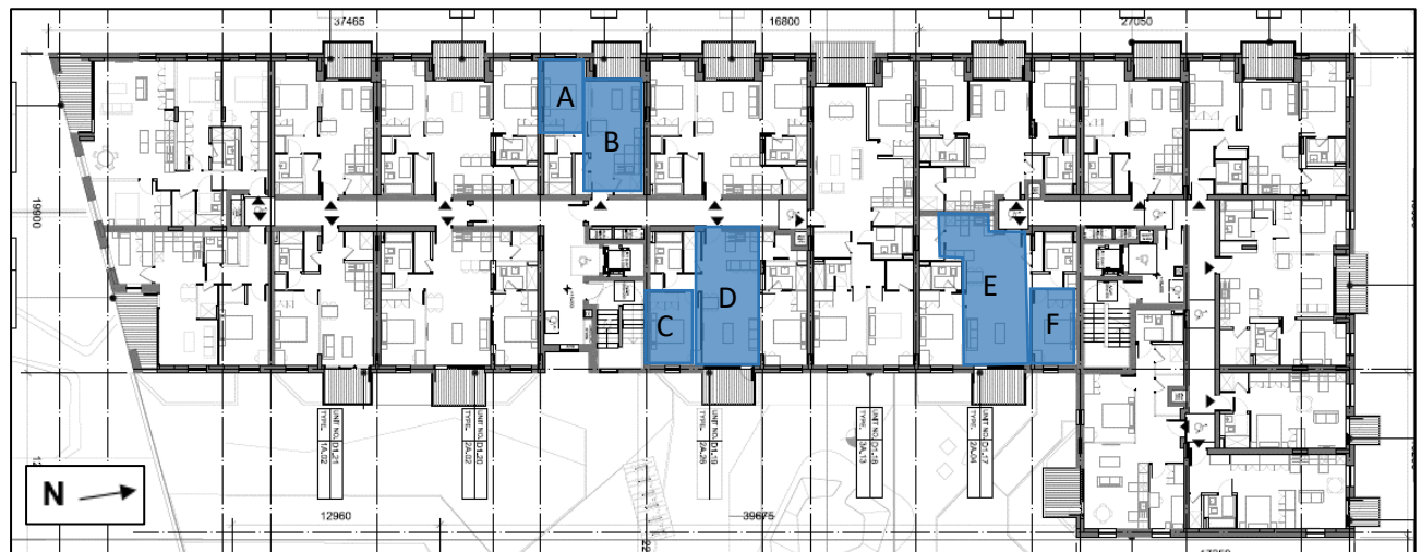
Figure 21 - Block D1 Level 02 - Assessed Rooms
