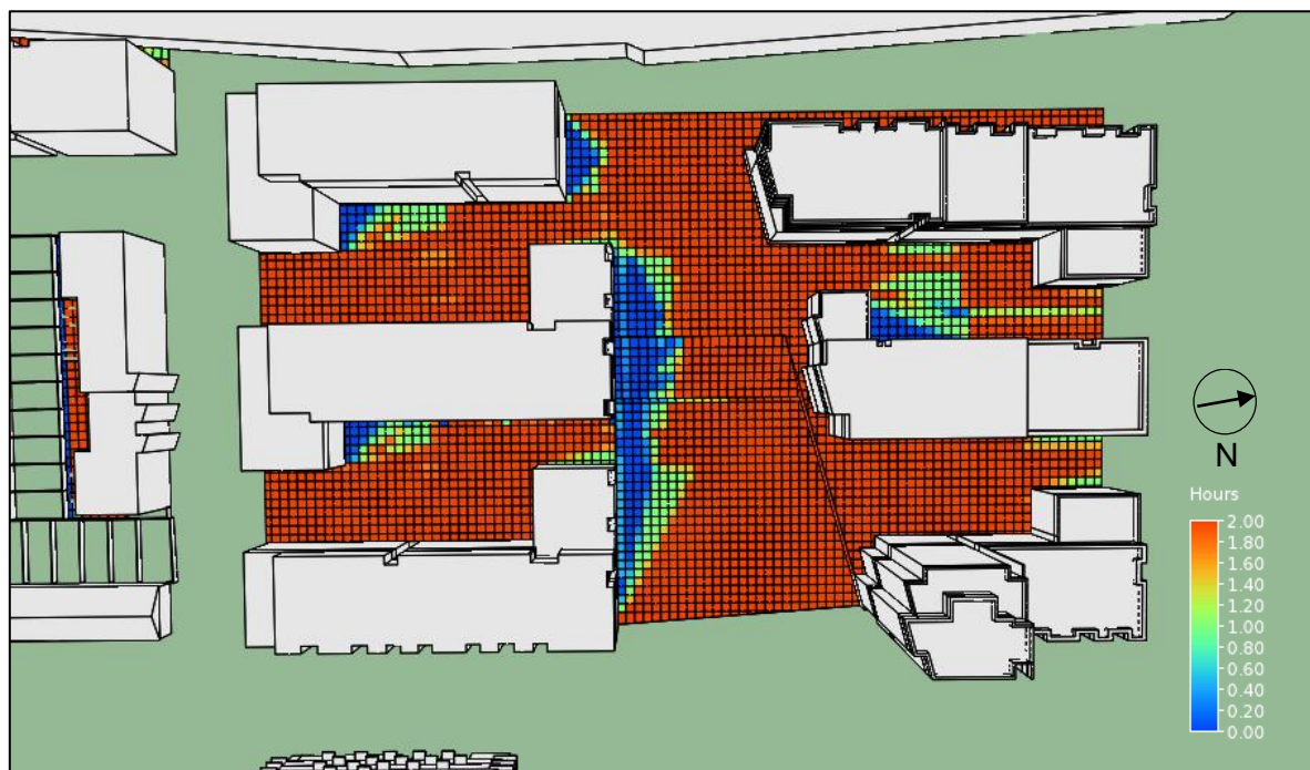
Figure 51– Communal amenity spaces to Stapolin Square – hours of sunlight on March 21 st 2
