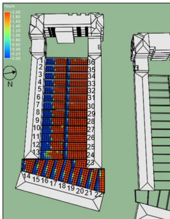
Figure 52 – Private amenity spaces to houses (Plot B4) – hours of sunlight on March 21 st 2
