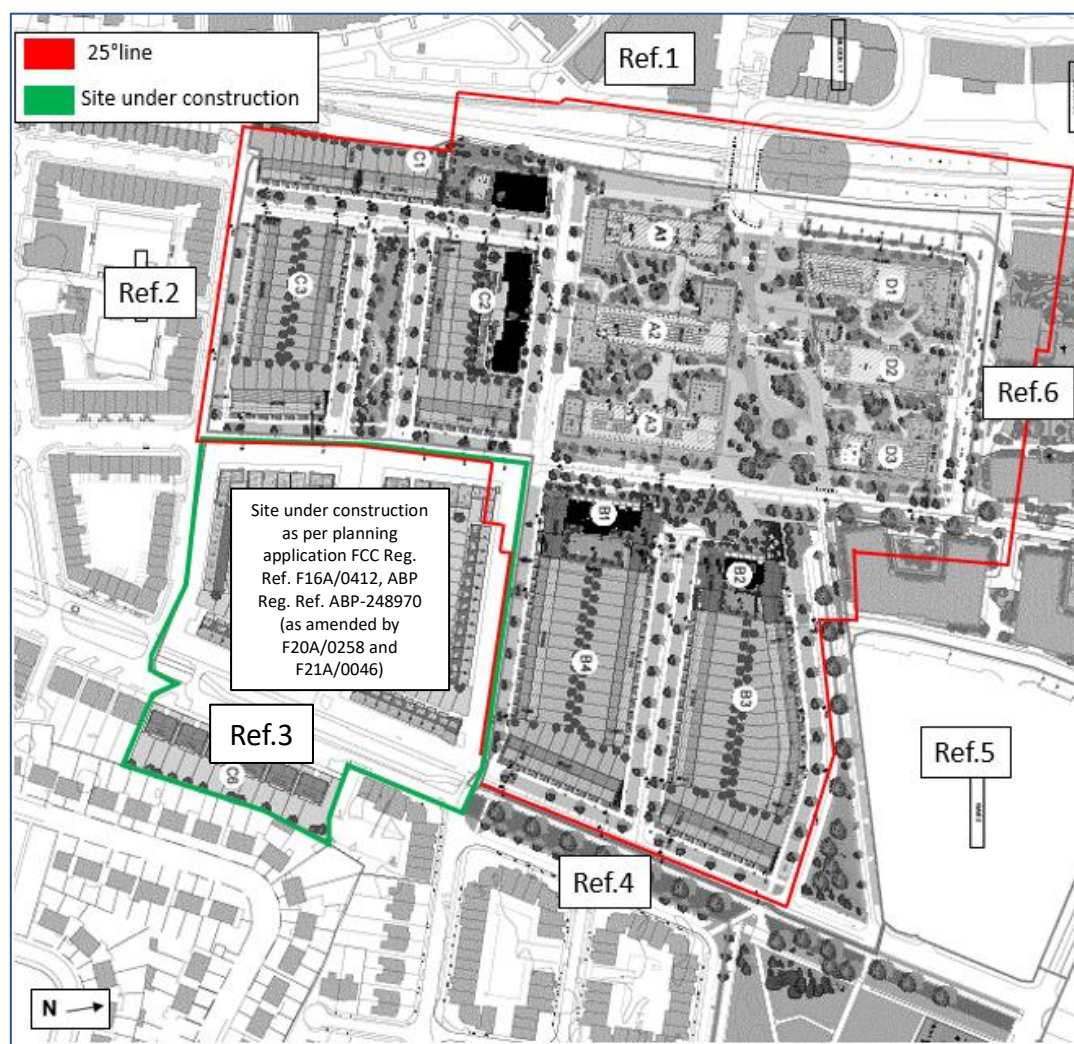
Figure 61 – 25° Line Adjacent Properties
