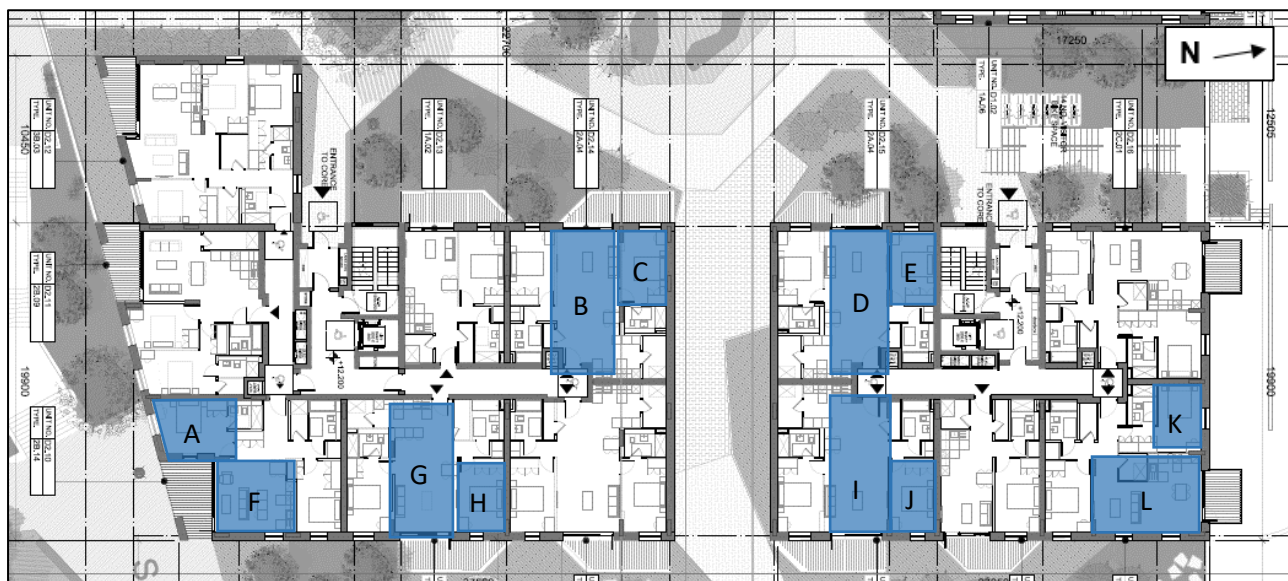
Figure 26 - Block D2 Level 01 - Assessed Rooms
