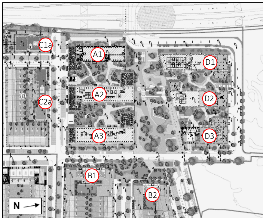
Figure 5 – Apartment Block Layout Plan
