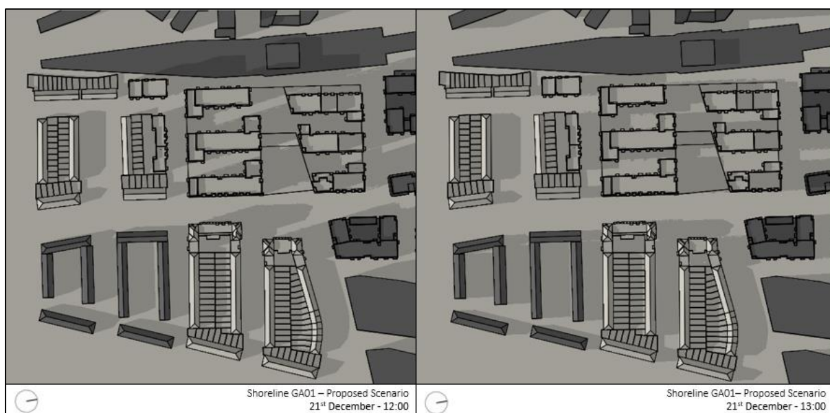
Figure 75 - Overshadowing image on December 21st at 12 p.m. and 1 p.m.
