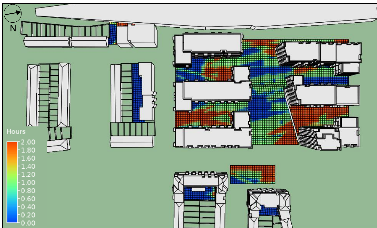
Figure 88 – Sunlight Analysis December 21 st
