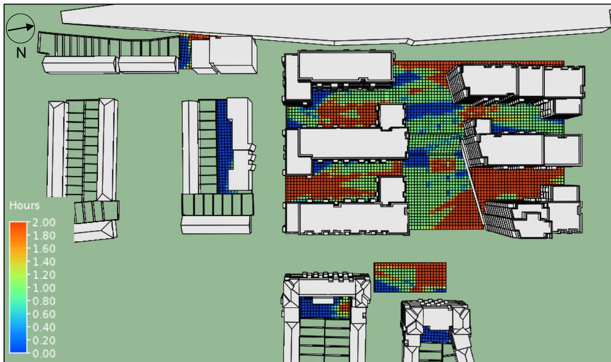
Figure 77 – Sunlight Analysis January 21 st
